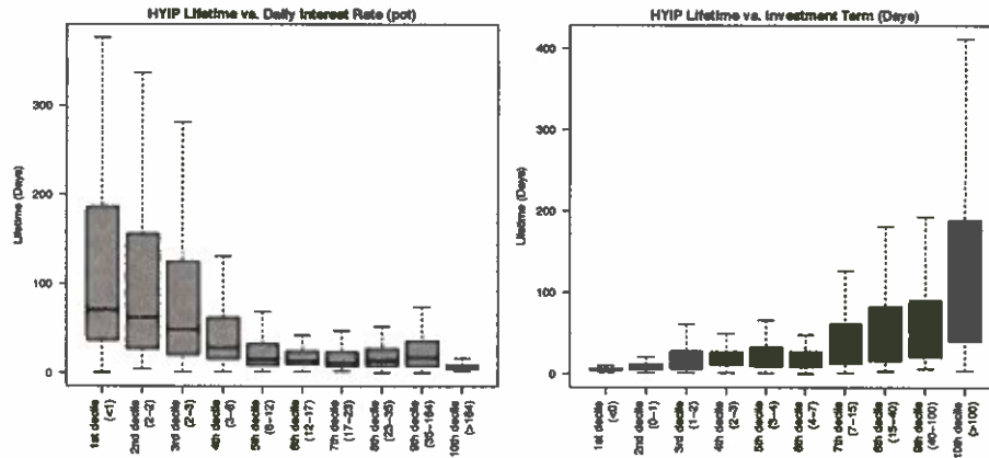
Fig. 3. HYIPs with lower daily interest rates tend to last longer before collapsing (left); HYIPs with longer mandatory investment periods tend to survive longer (right).
